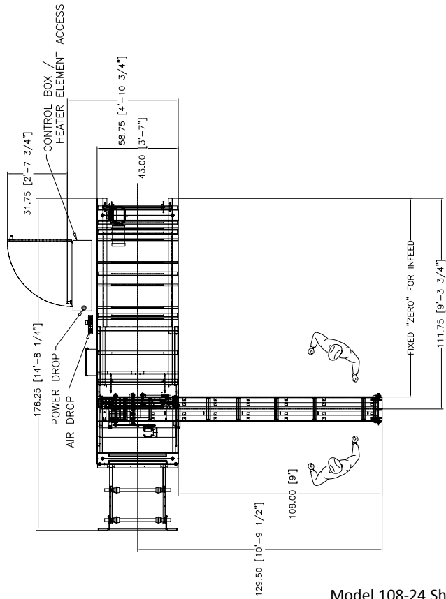
Model 108-24 Shown
