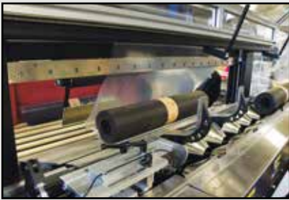
108-70 Infeed Conveyor
